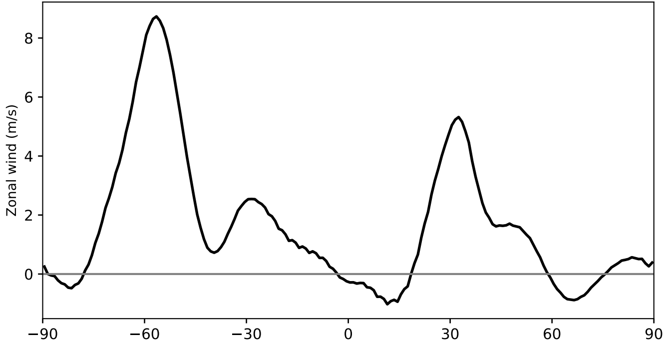
Model - Observations
