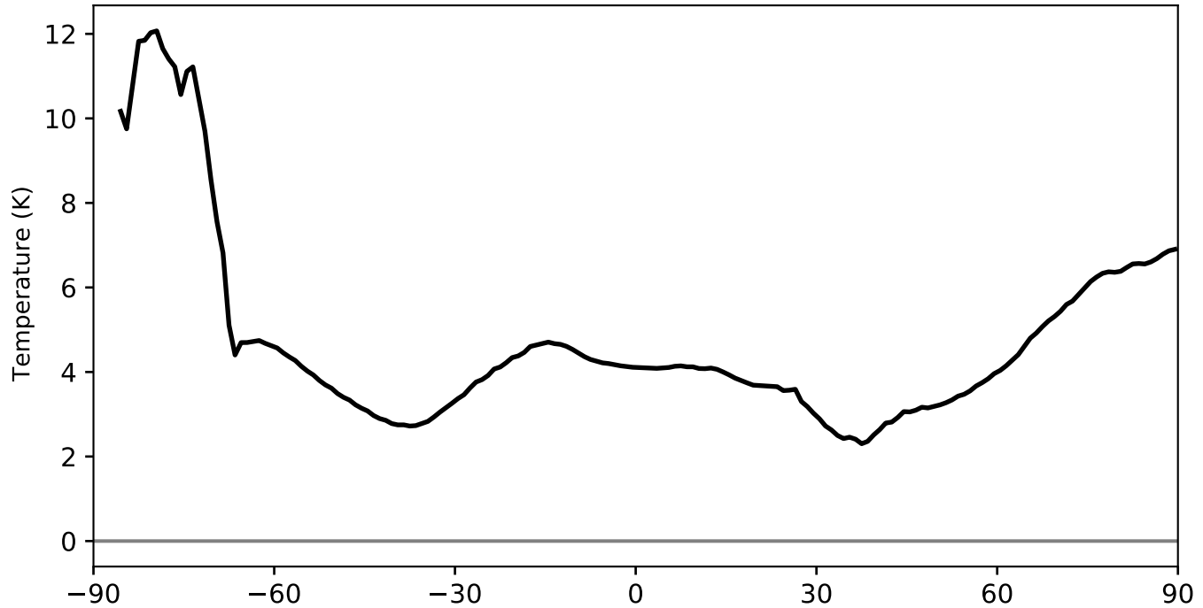
Model - Observations
