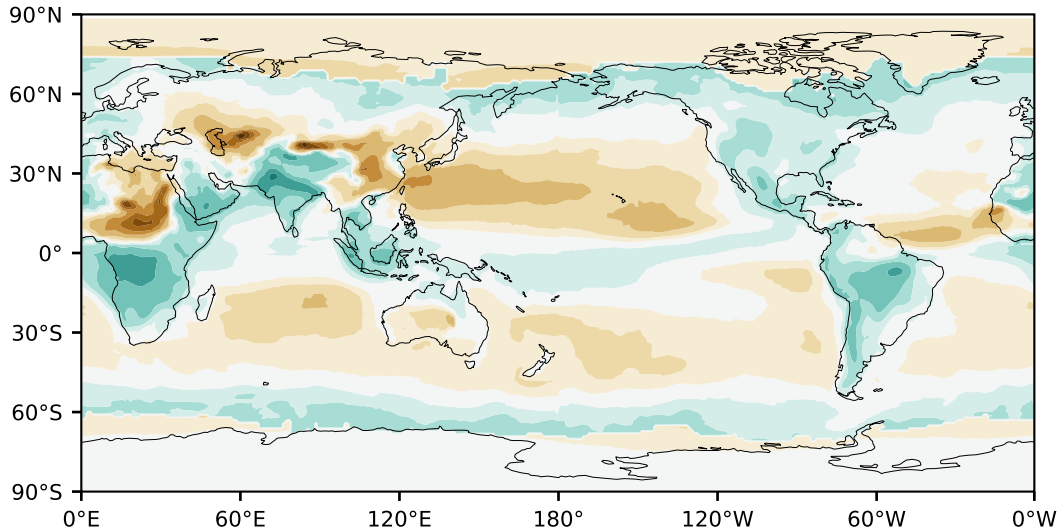
Model - Observations
