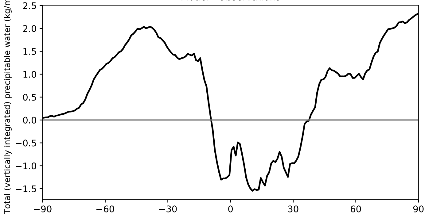
Model - Observations
