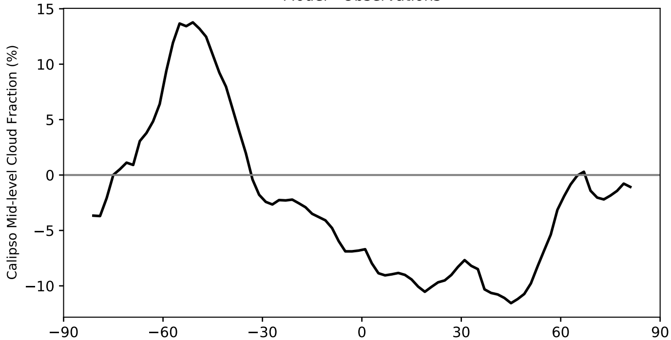
Model - Observations
