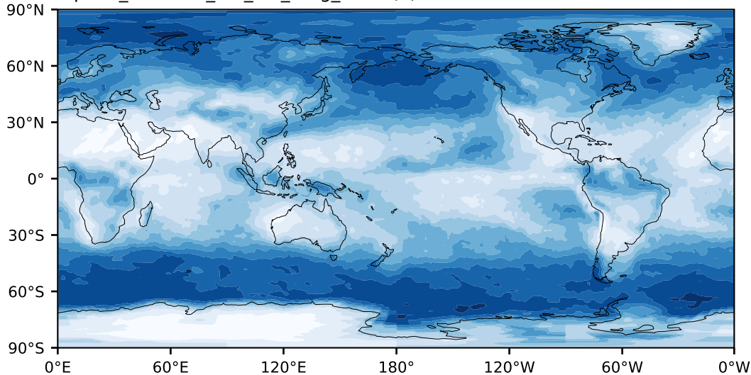
alpha3_min10nc_tk1_ZM_berg_GWD (3)
