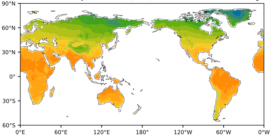
CRU Global Monthly Mean T Land (None)
