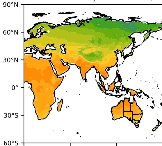
CRU Global Monthly Mean T Land (None)
