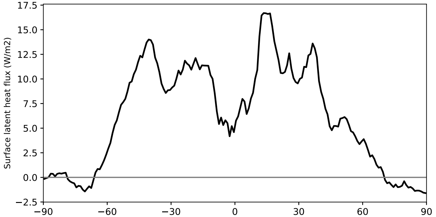
Model - Observations
