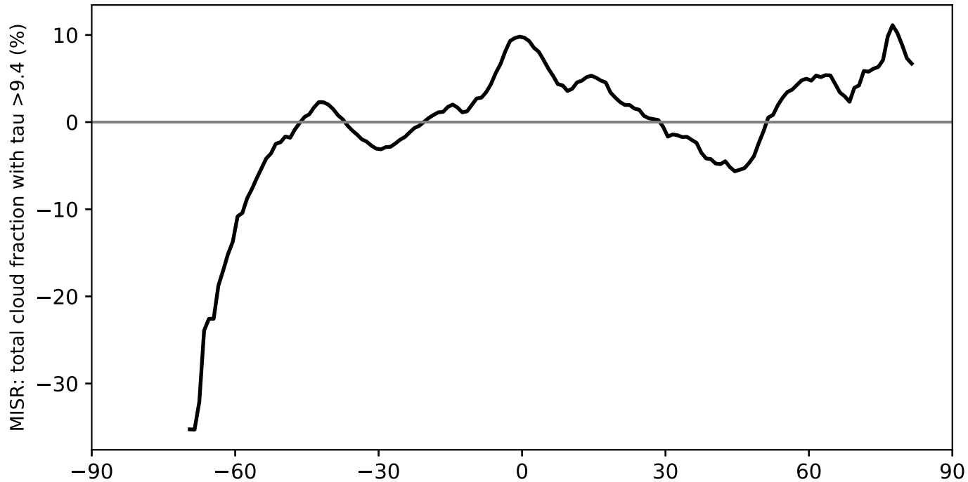
Model - Observations
