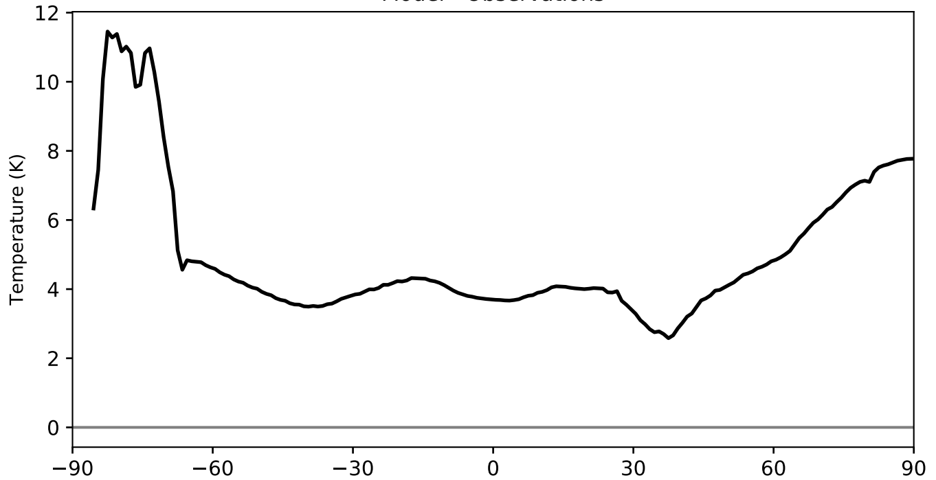
Model - Observations
