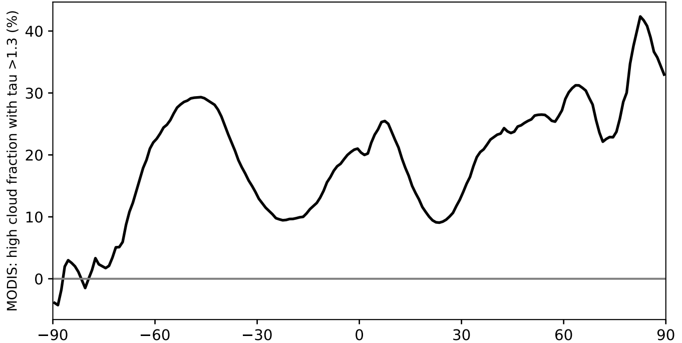
Model - Observations
