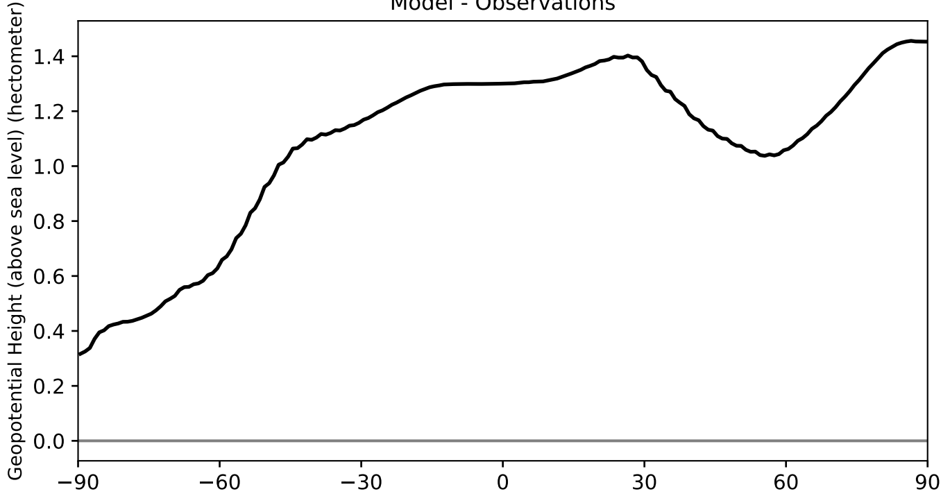
Model - Observations
