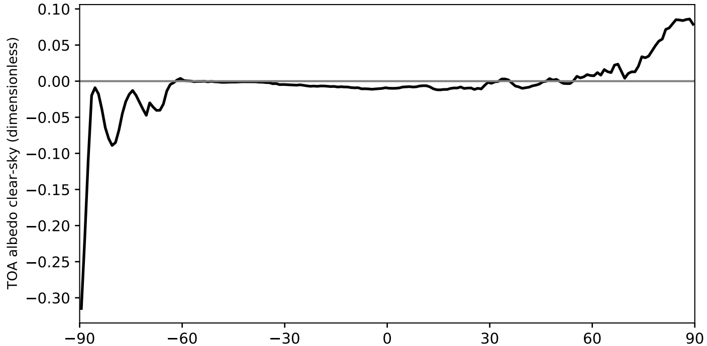
Model - Observations
