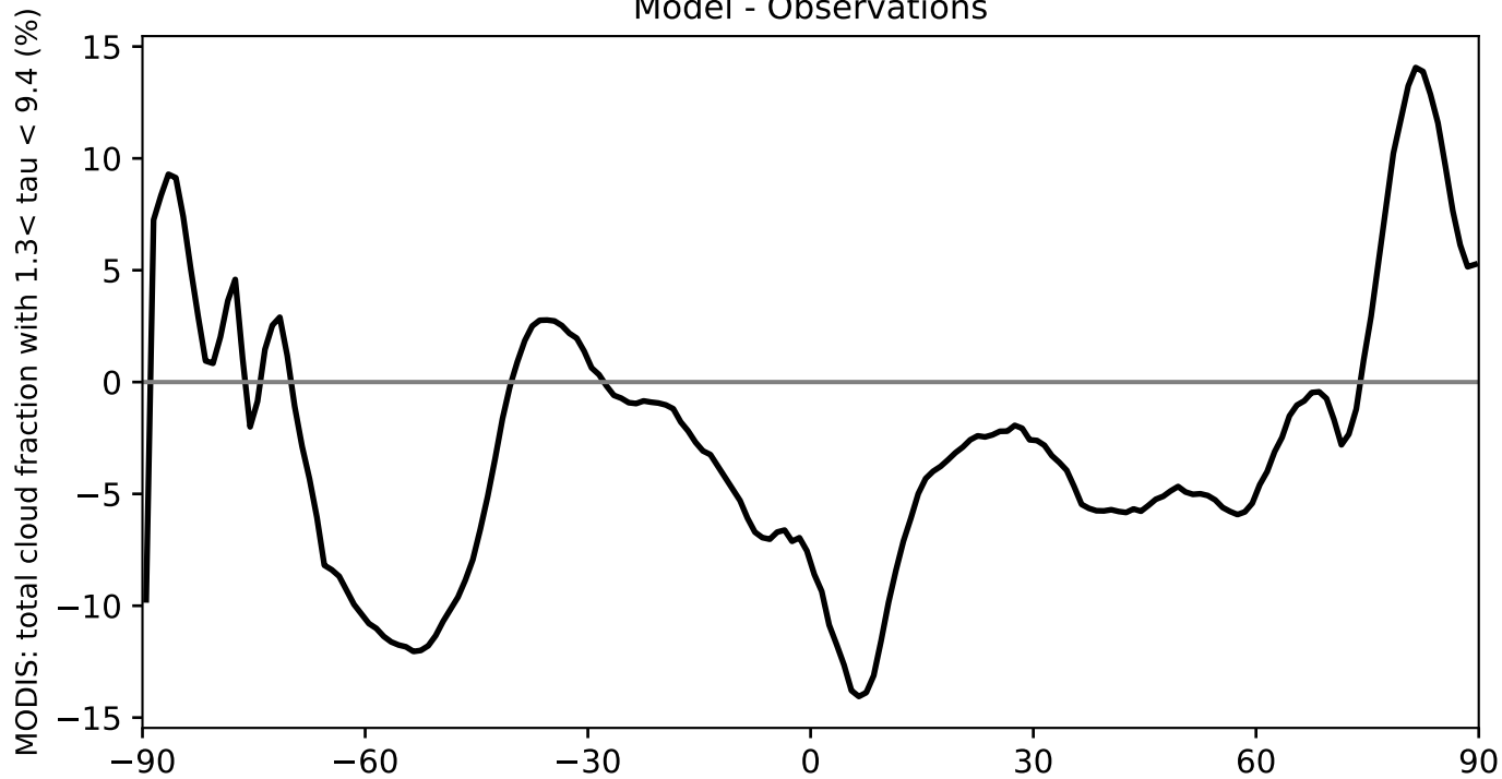
Model - Observations
