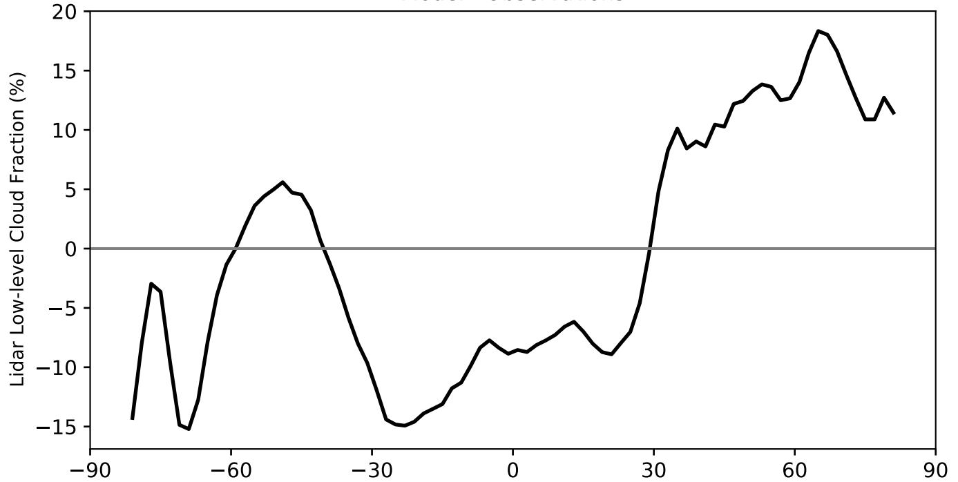
Model - Observations
