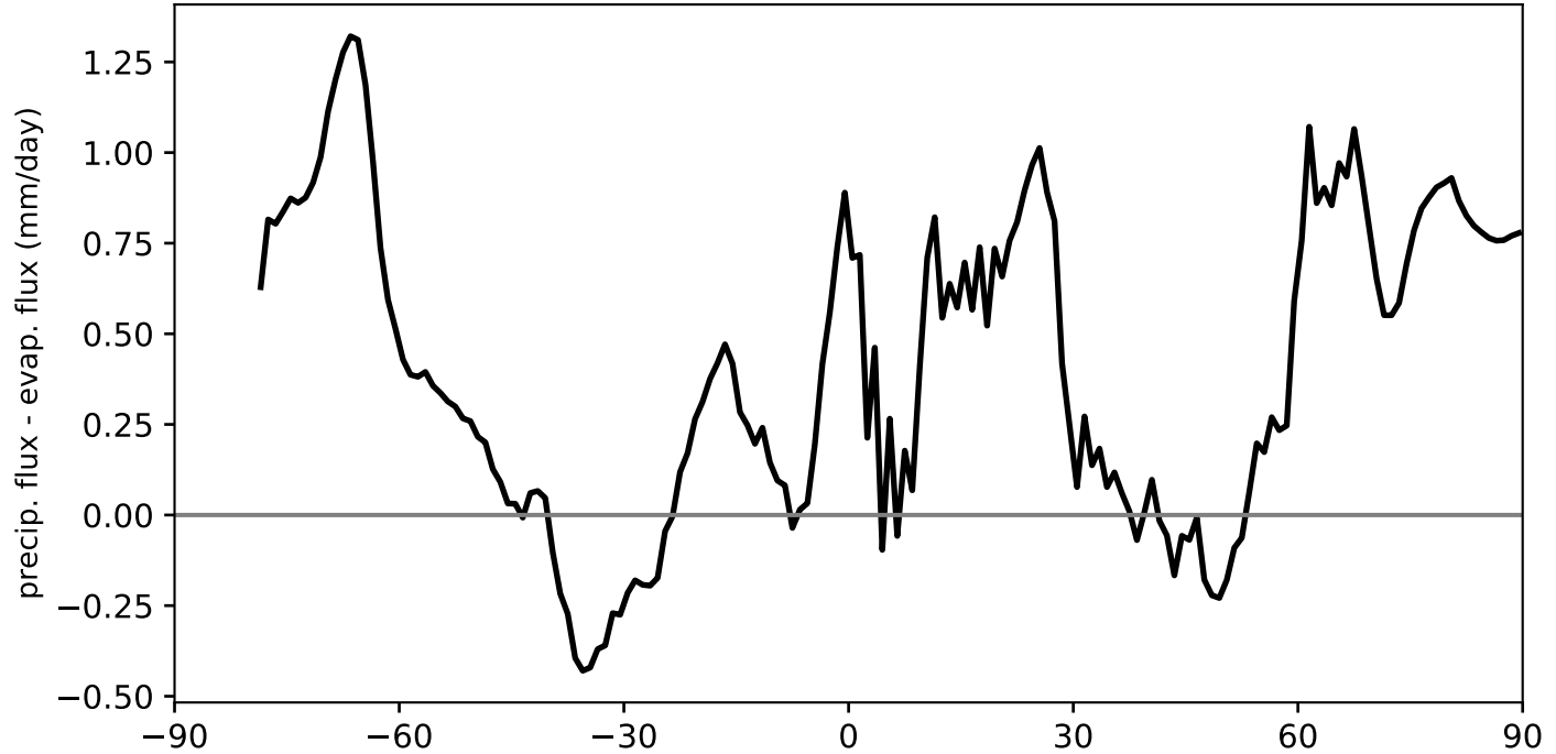
Model - Observations
