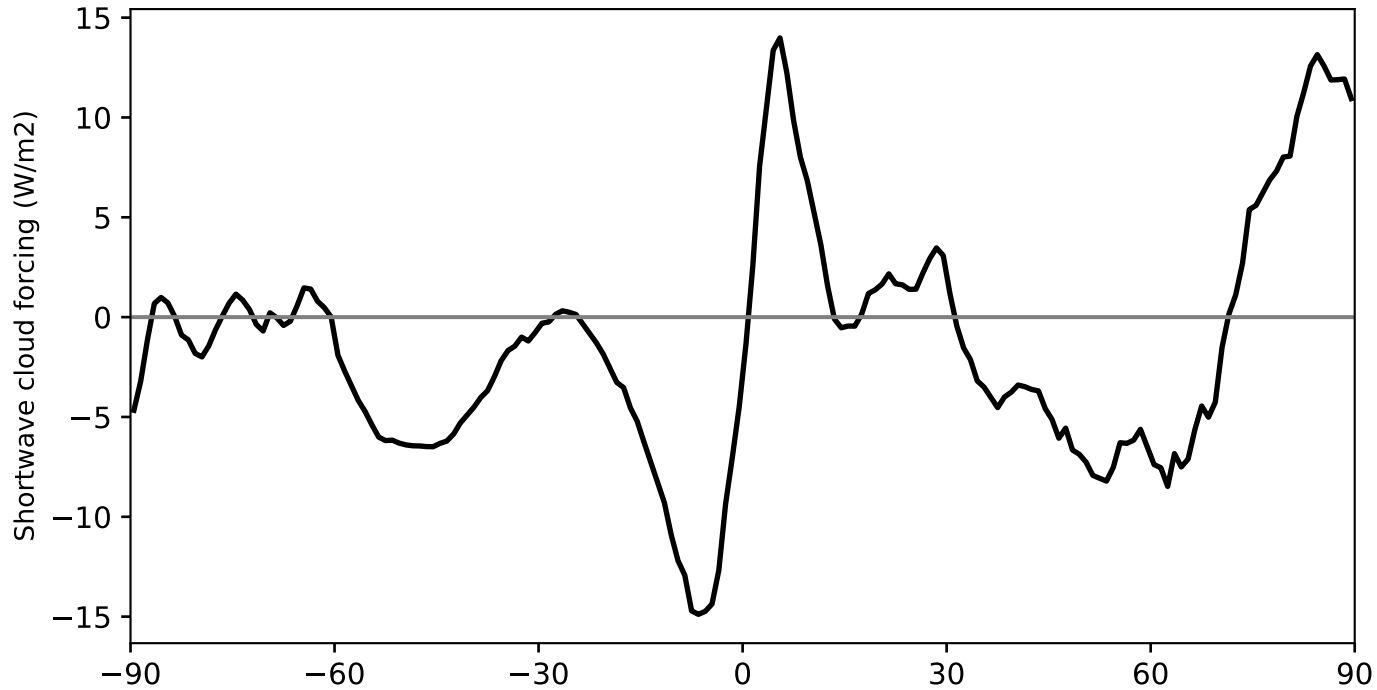
Model - Observations
