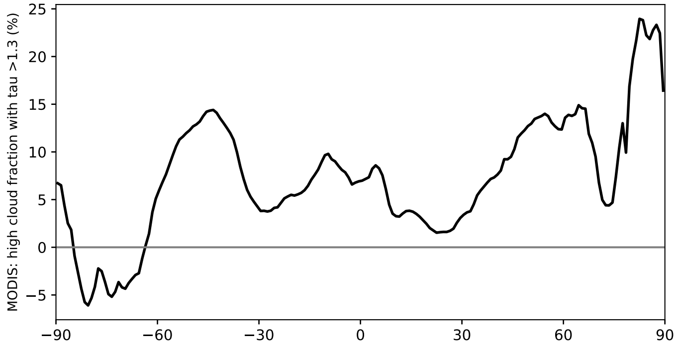
Model - Observations
