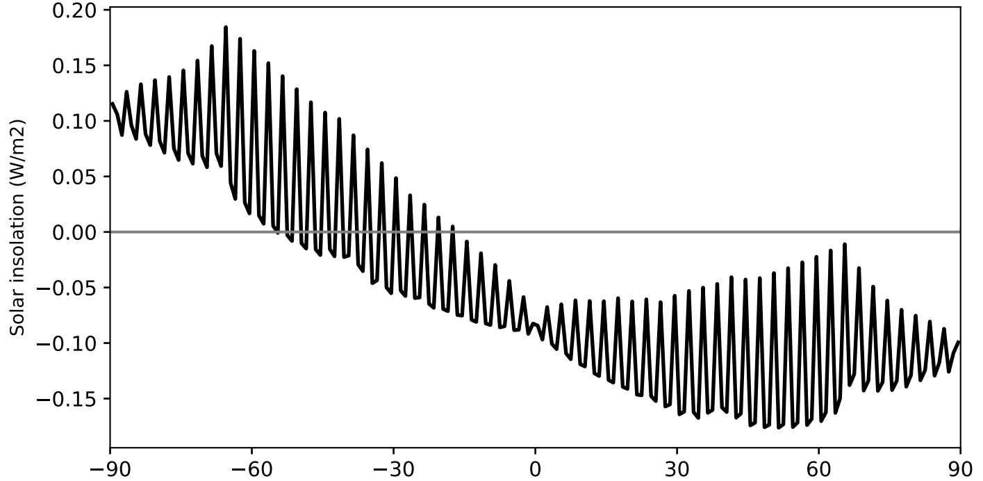
Model - Observations
