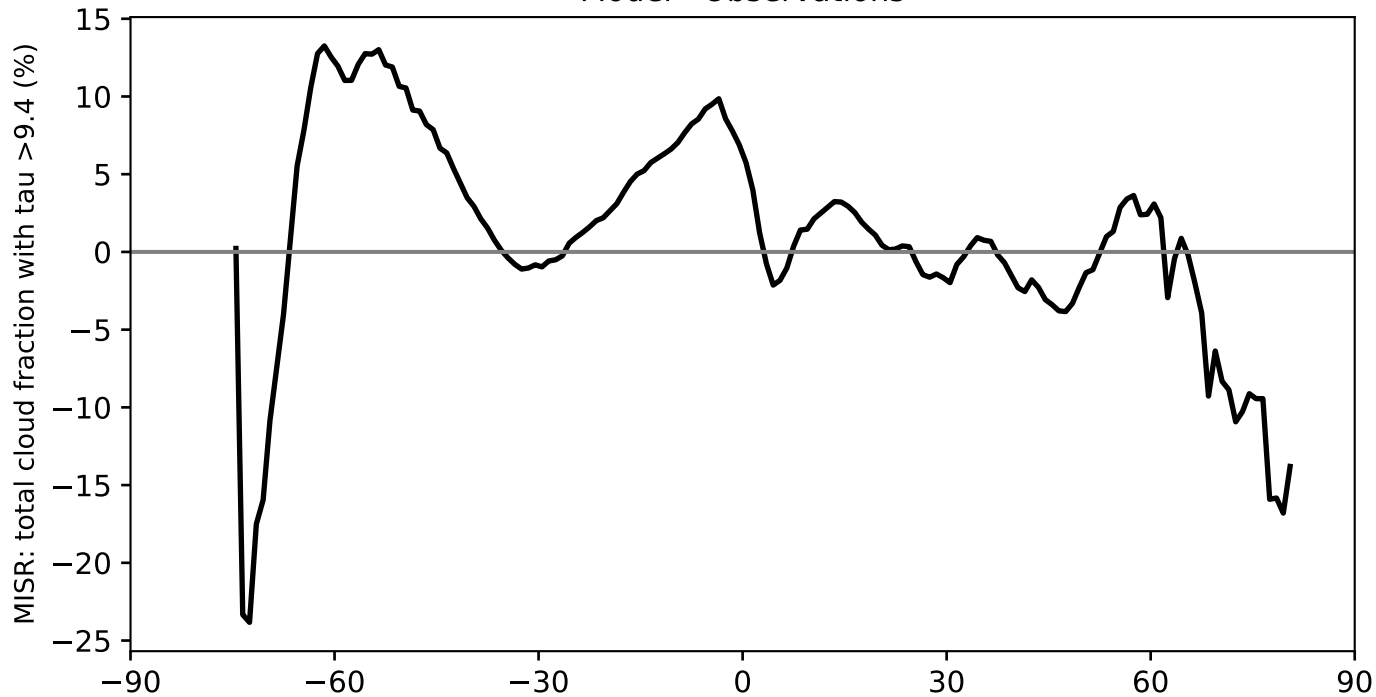
Model - Observations
