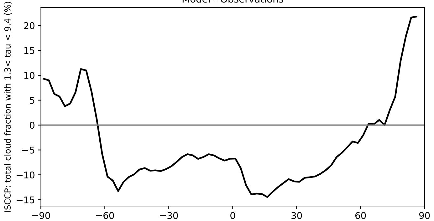
Model - Observations
