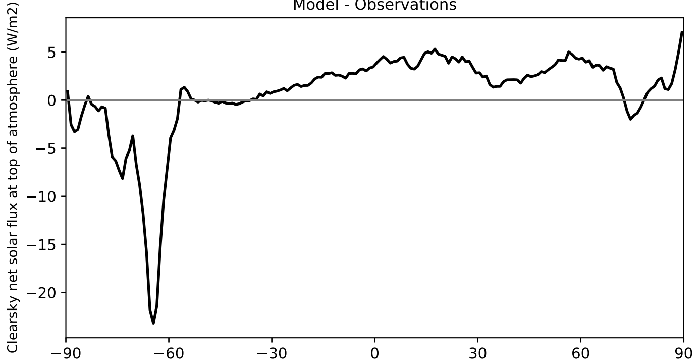
Model - Observations
